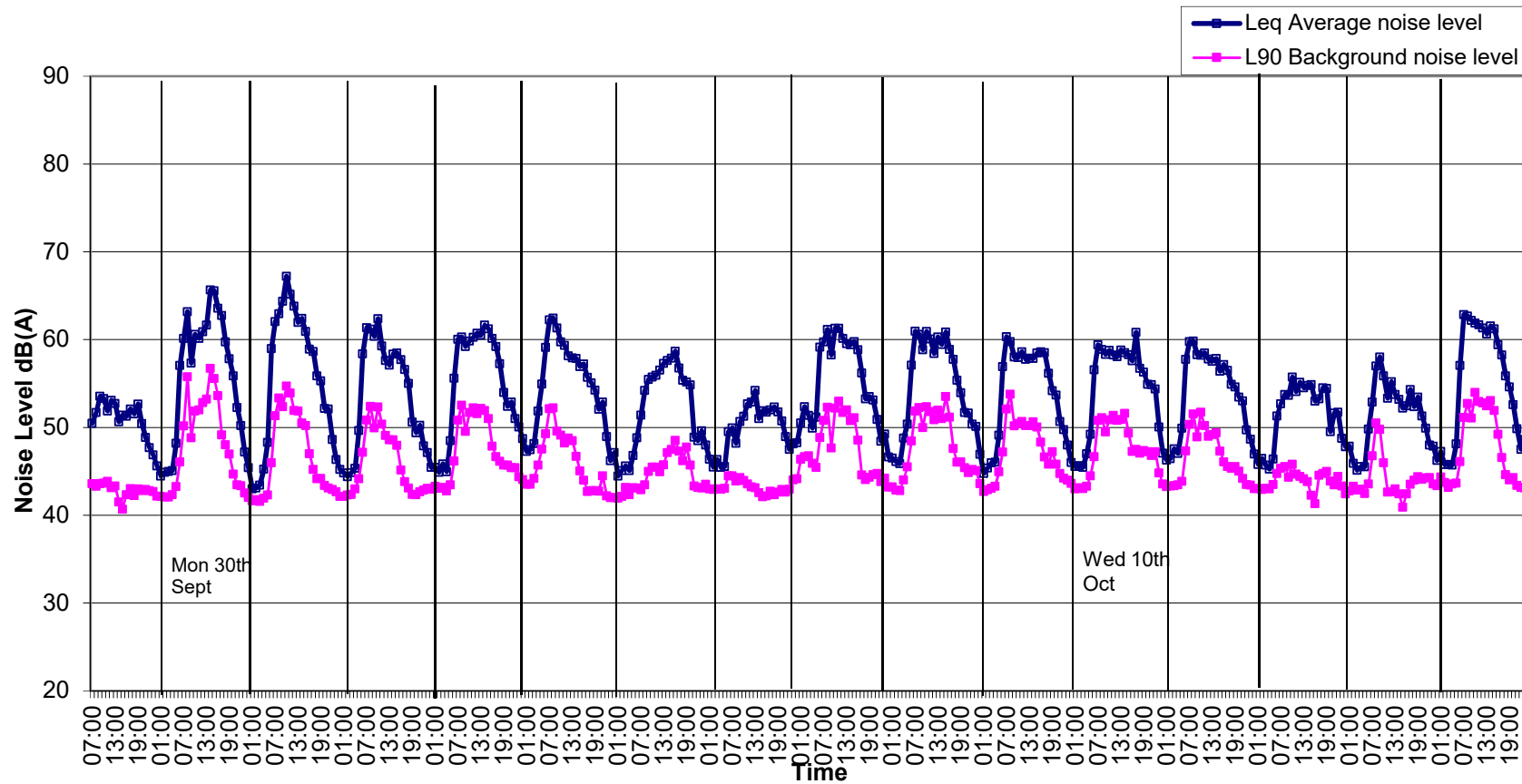
Graph 1: Noise Levels at Location A East Quad West Boundary Wall from 29 th September to 14 th October 2019.
