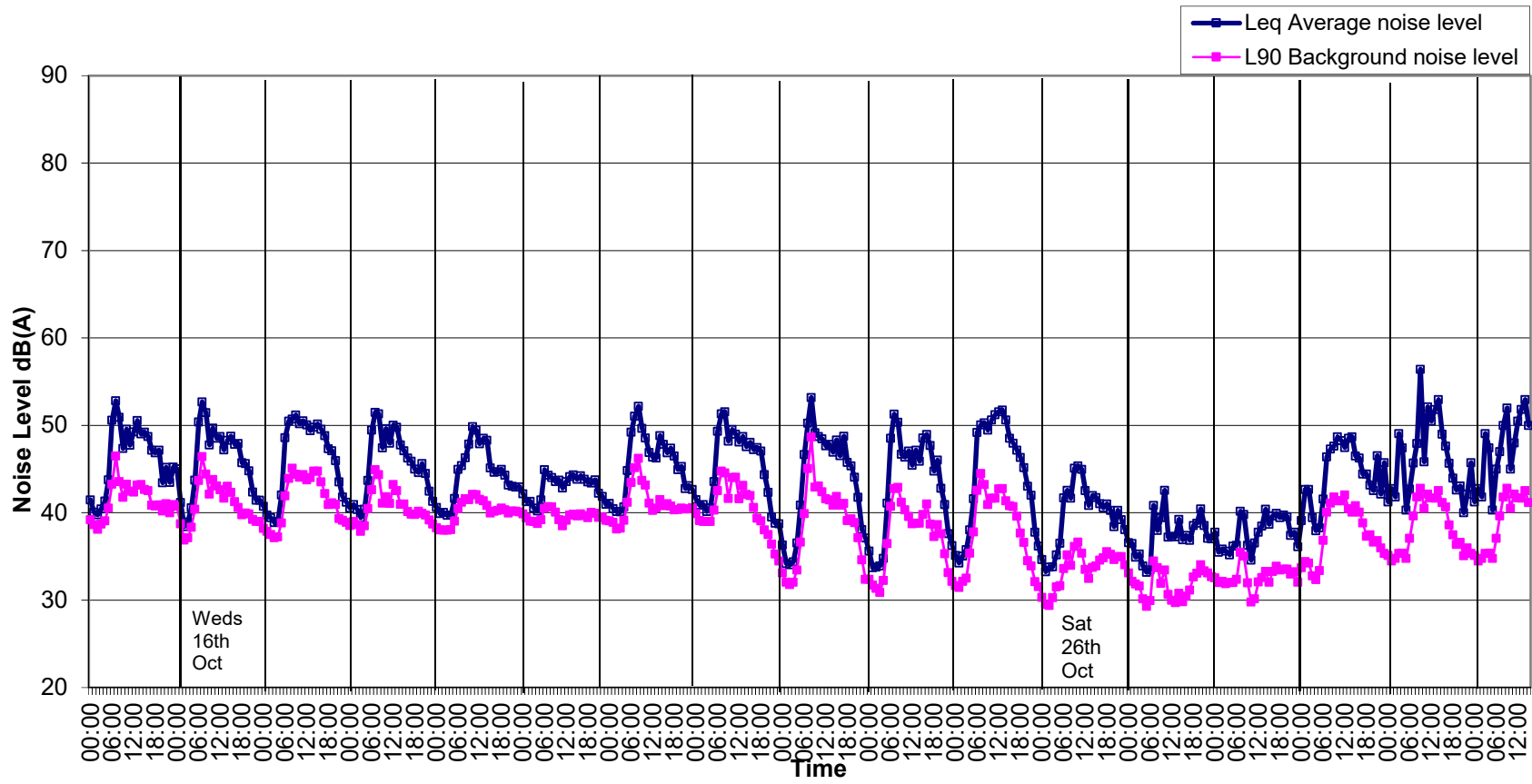
Graph 4: Noise Levels at Location B Grangegorman Upper from 14 th to 31 st October 2019.
