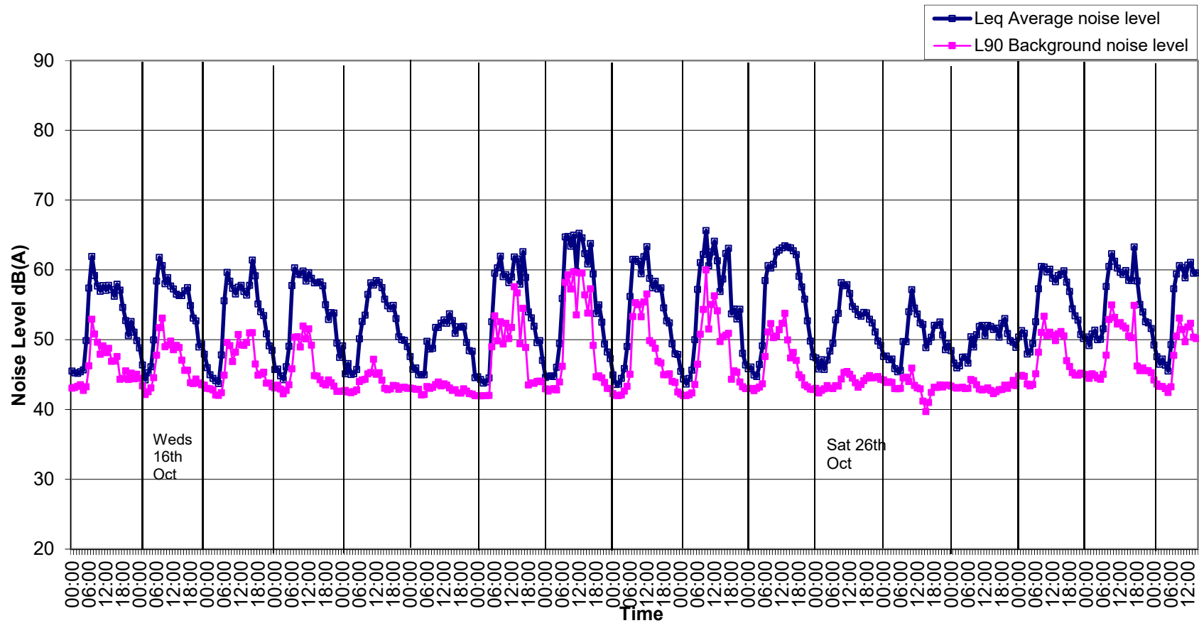
Graph 2: Noise Levels at Location A East Quad West Boundary Wall from 14 th to 31 st October 2019.
