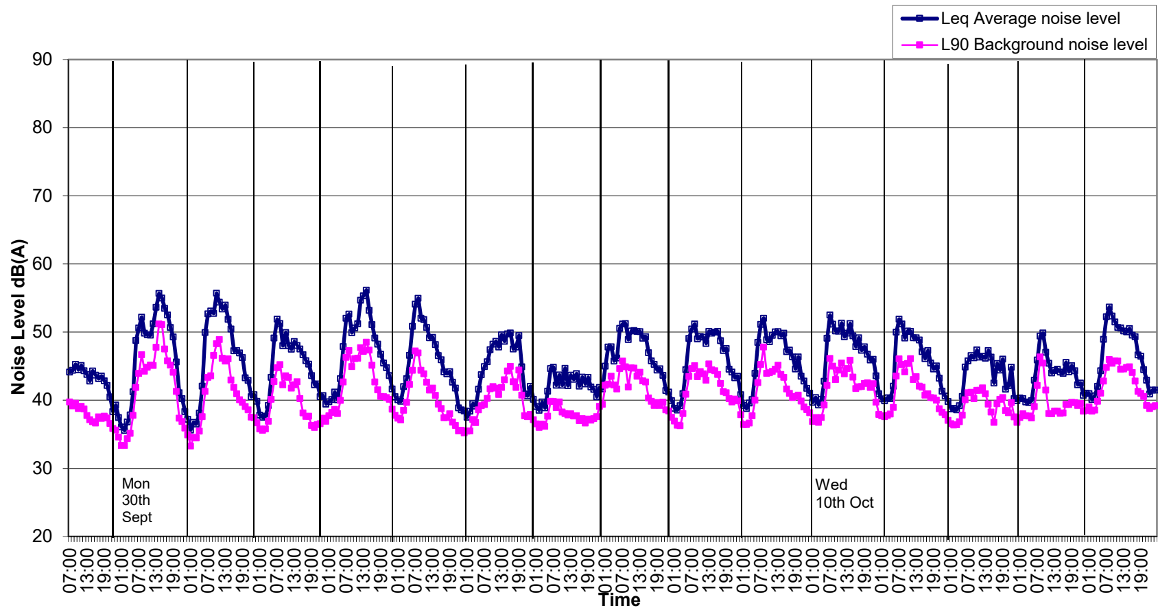
Graph 3: Noise Levels at Location B Grangegorman Upper from 29 th September to 14 th October 2019.
