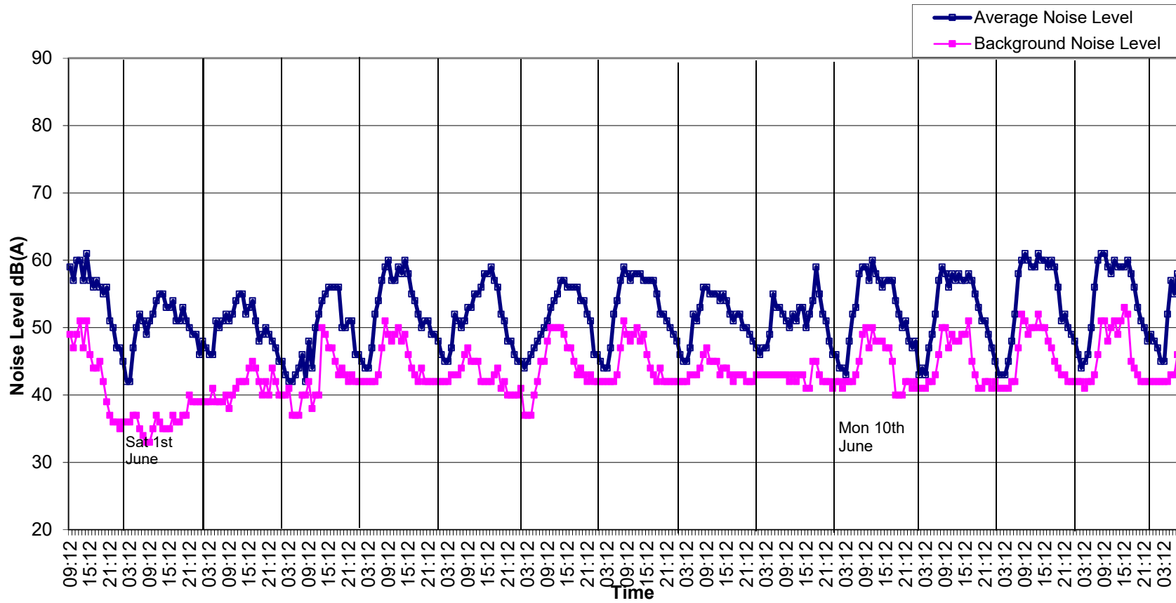
Graph 1: Noise Levels at Location A East Quad West Boundary Wall from 31 st May to 14 th June 2019.
