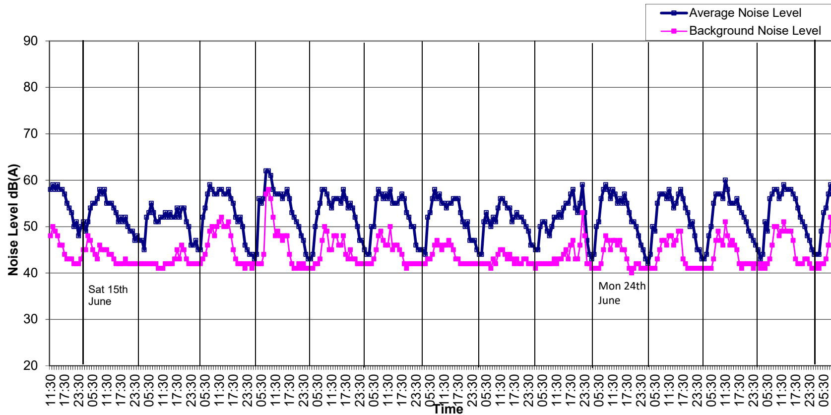
Graph 4: Noise Levels at Location B Grangegorman Upper from 14 th to 28 th June 2019.
