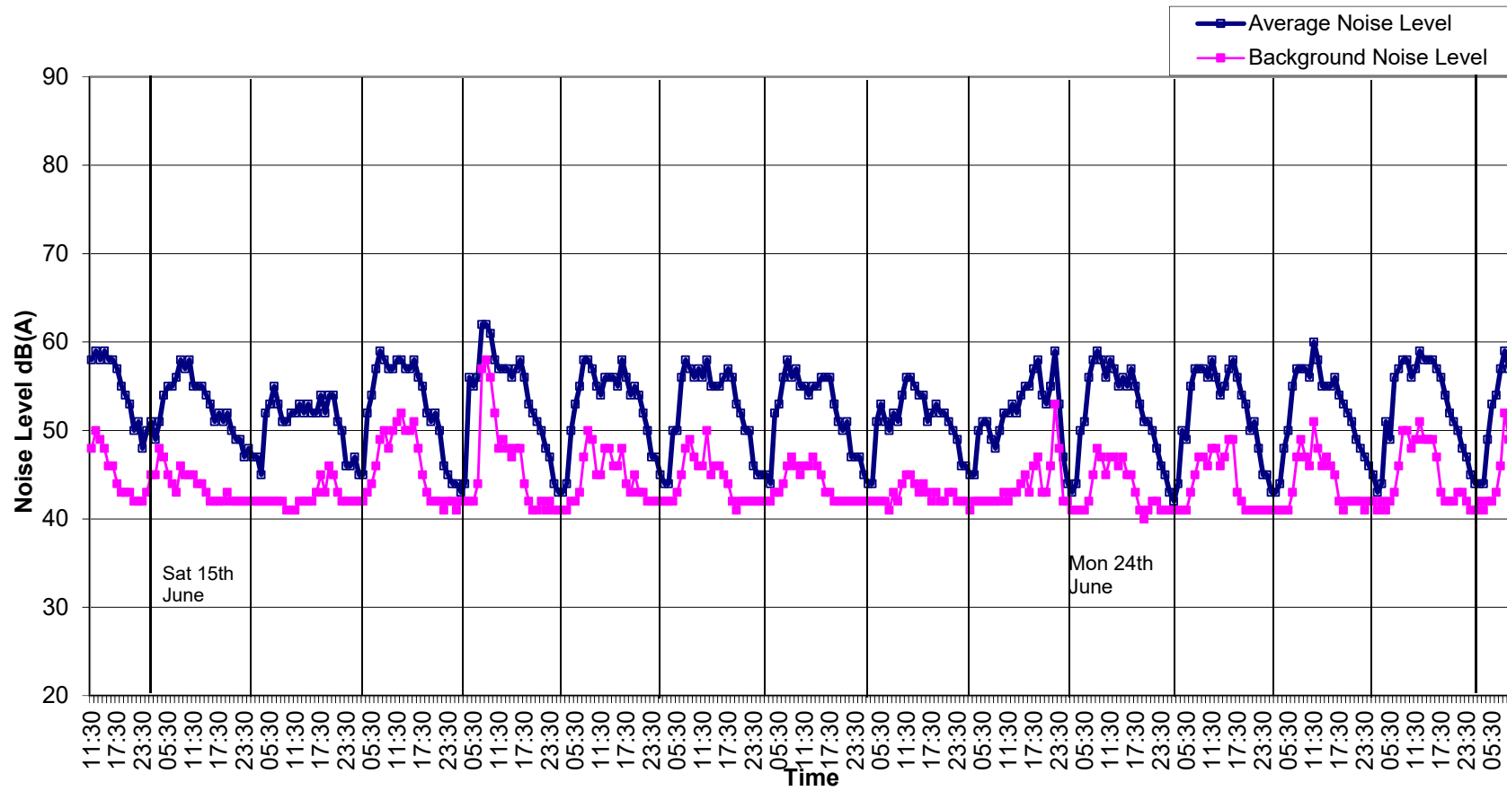
Graph 2: Noise Levels at Location A East Quad West Boundary Wall from 14 th to 28 th June 2019.
