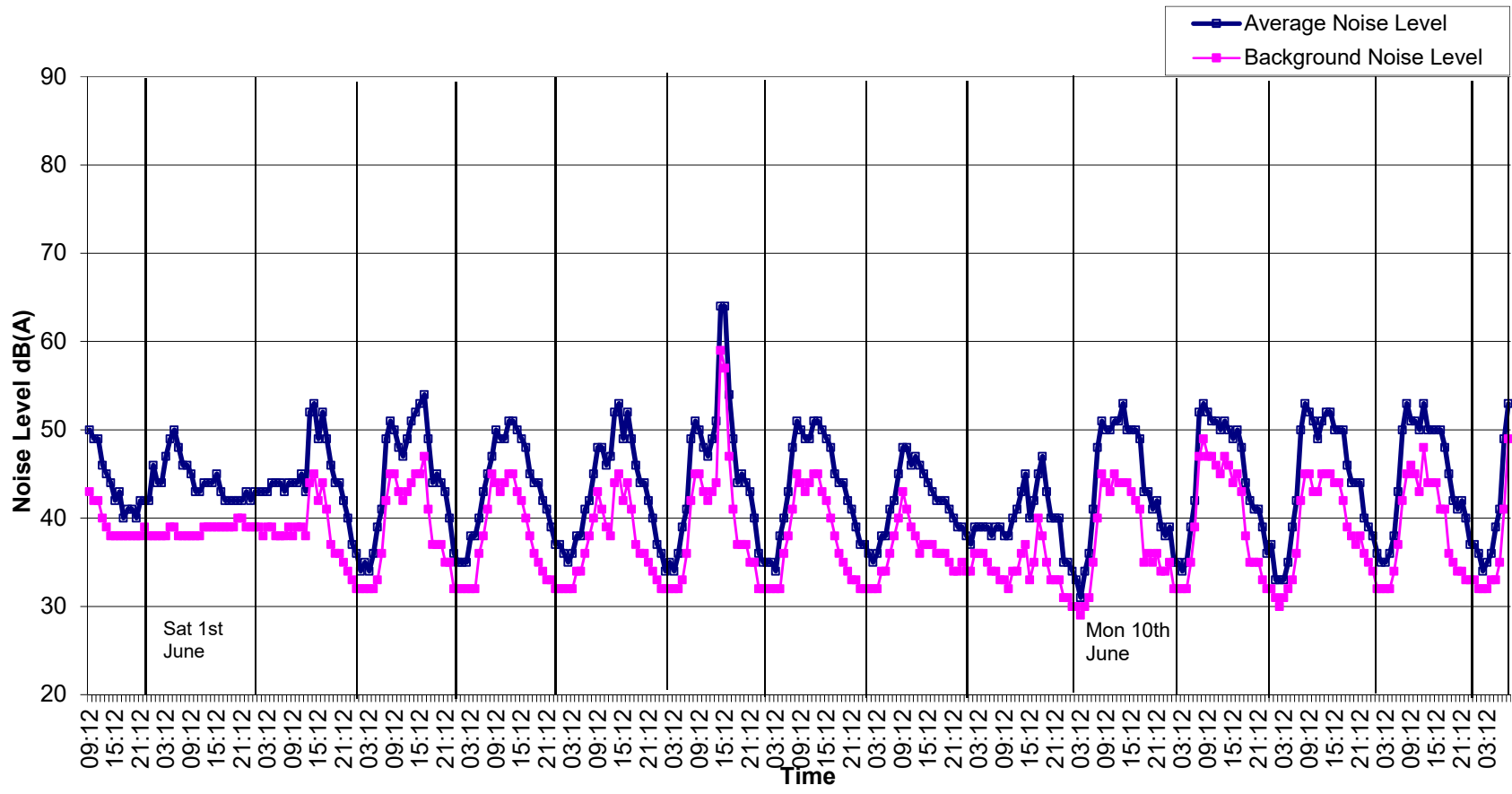
Graph 3: Noise Levels at Location B Grangegorman Upper from 31 st May to 14 th June 2019.
