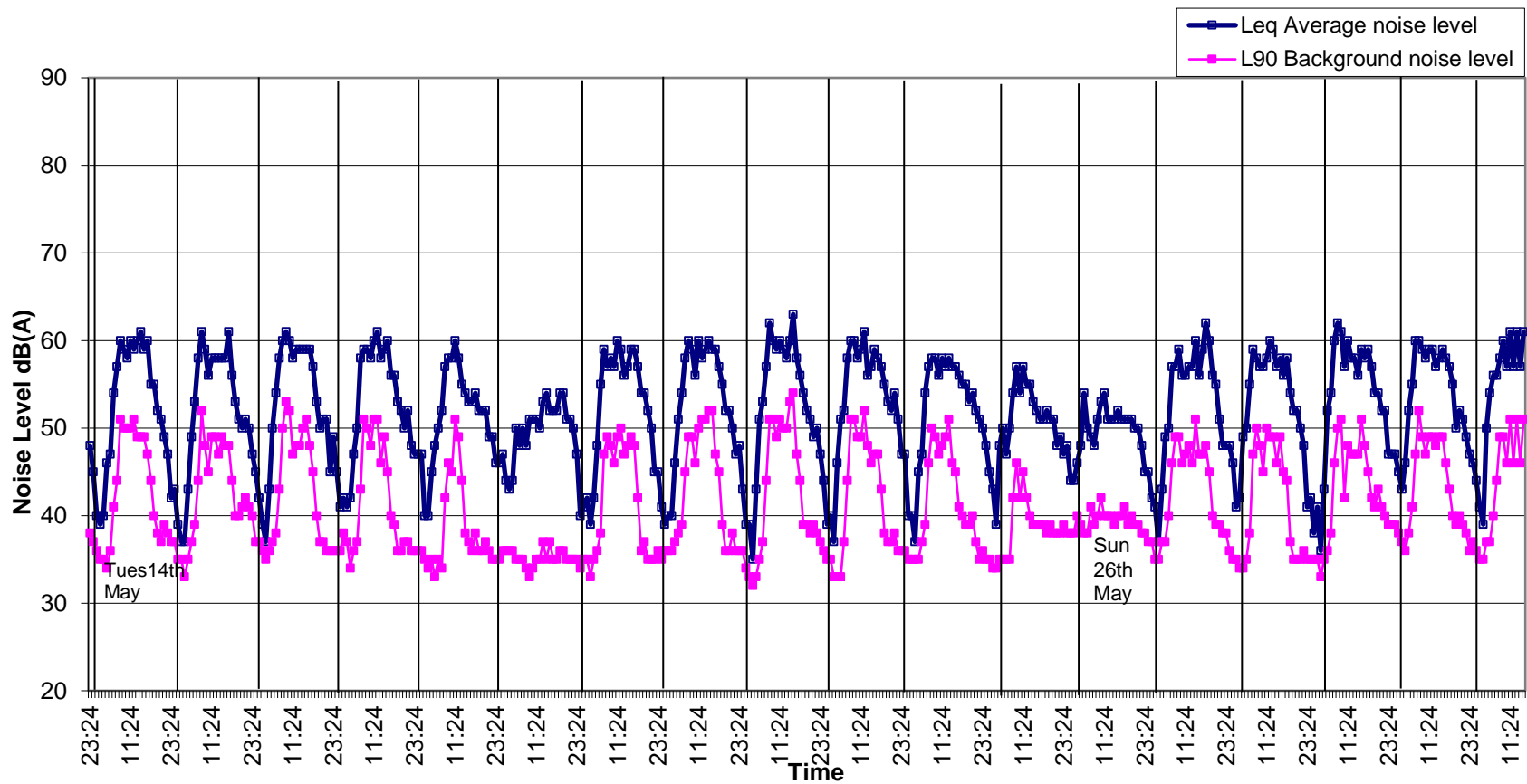
Graph 2: Noise Levels at Location A East Quad West Boundary Wall from 13 th to 31 st May 2019.
