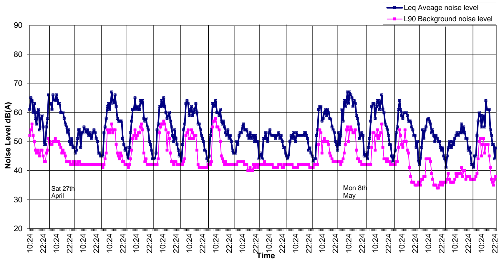
Graph 1: Noise Levels at Location A East Quad West Boundary Wall from 26 th April to 13 th May 2019.
