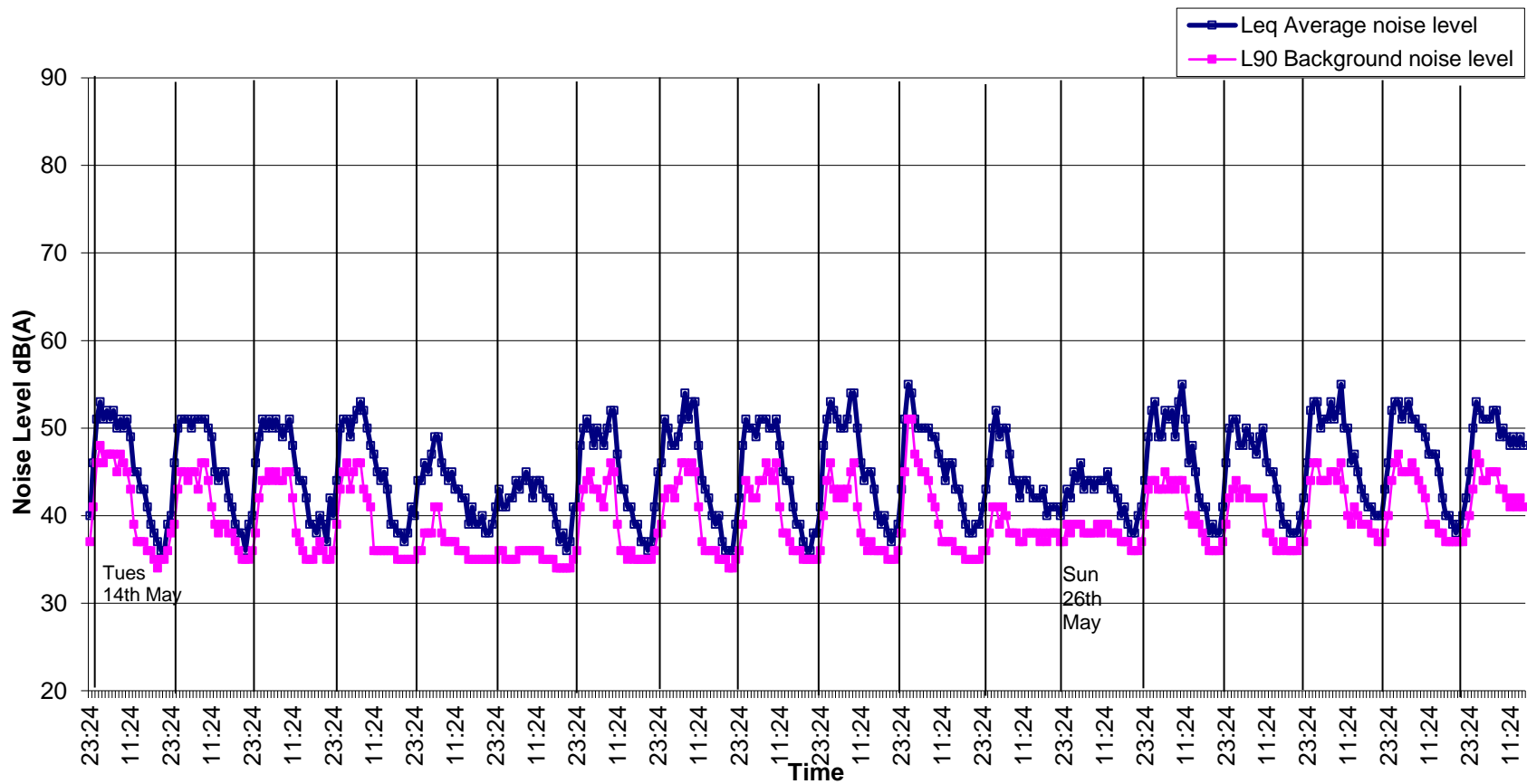
Graph 4: Noise Levels at Location B Grangegorman Upper from 13 th to 31 st May 2019.
