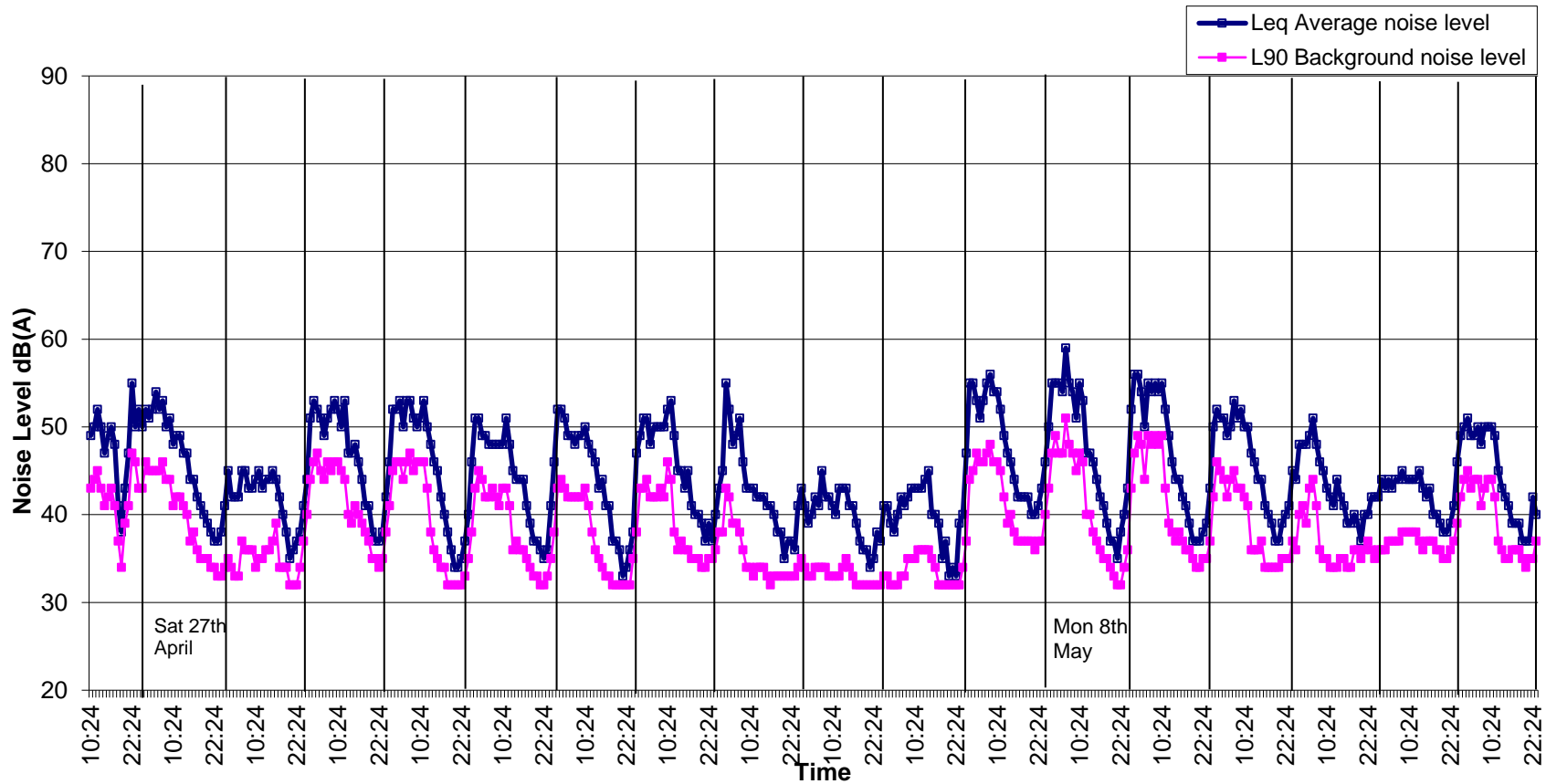
Graph 3: Noise Levels at Location B Grangegorman Upper from 26 th April to 13 th May 2019.
