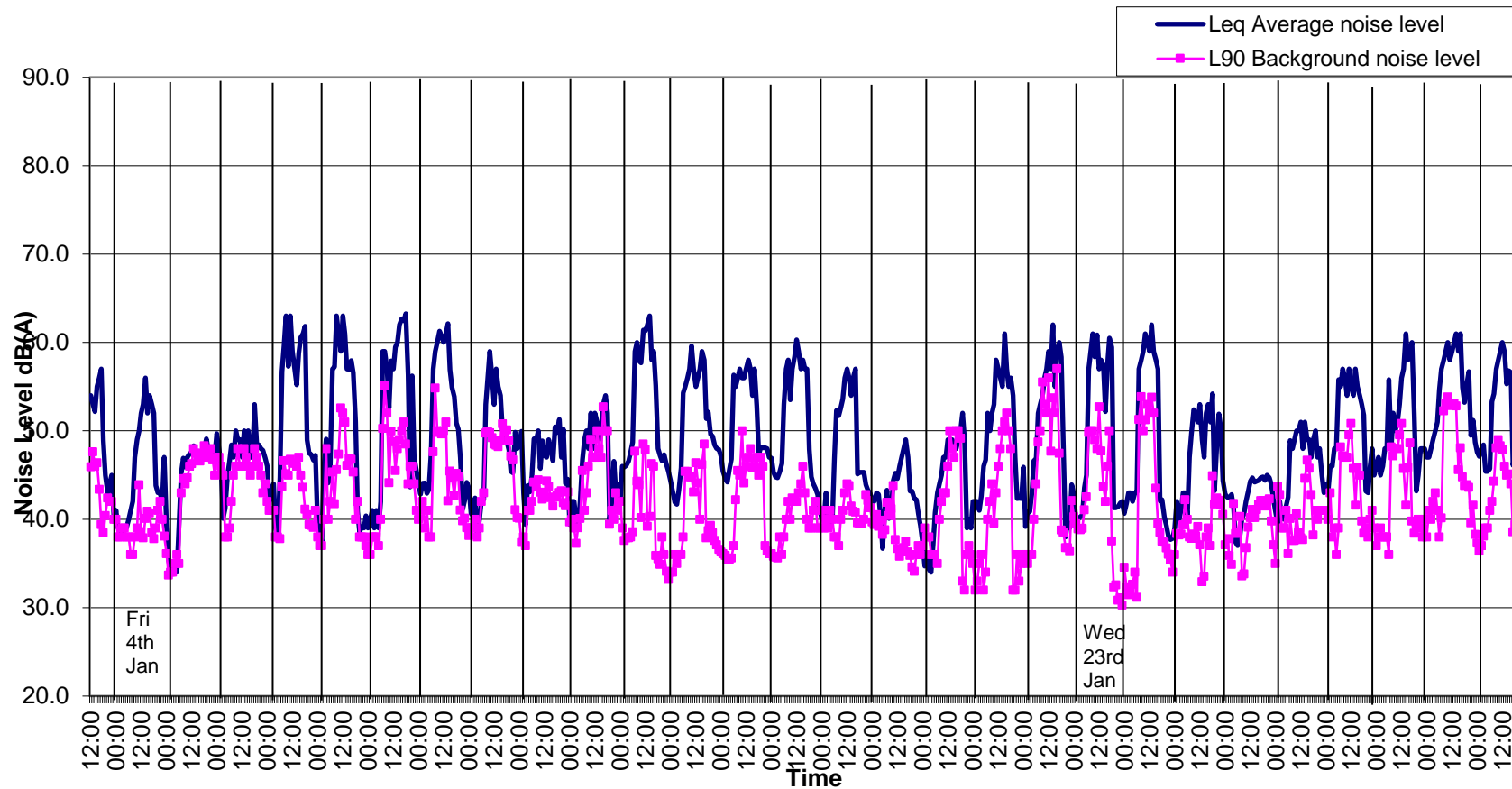
Graph 1: Noise Levels at Location A East Quad West Boundary Wall from 3 rd to 31 st January
