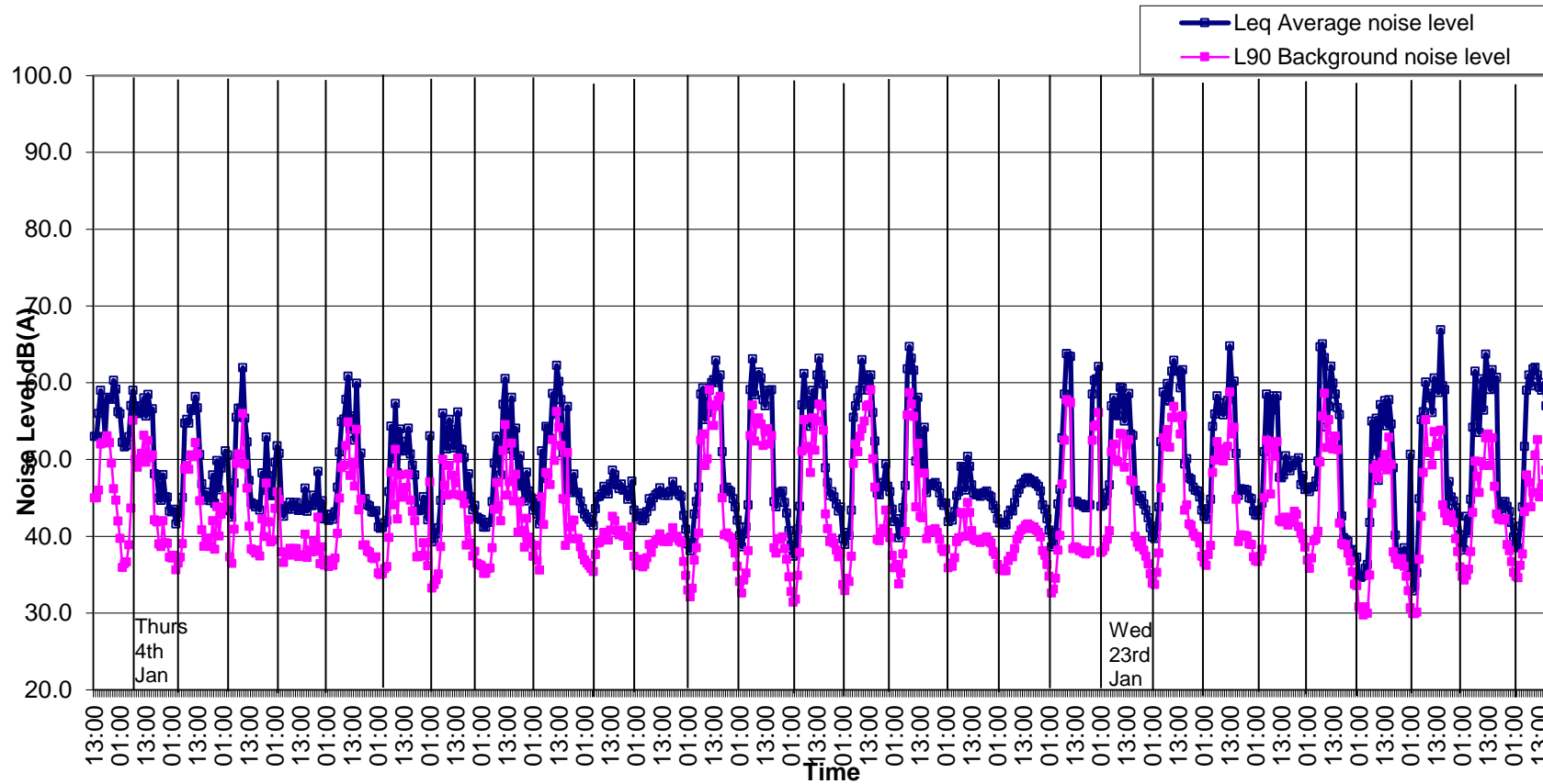
Graph 3: Noise Levels at Location B Grangegorman Upper from 3rd to 31st January.
