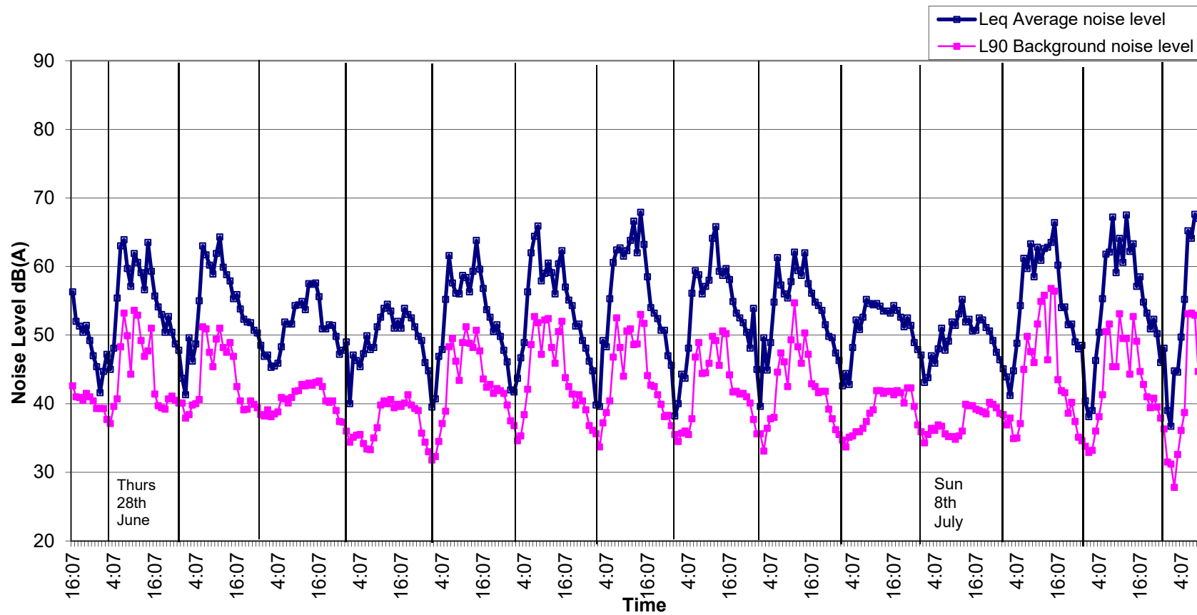
Graph 1: Noise Levels at Location A East Quad West Boundary Wall from 27 th June to 11 th July 2018.
