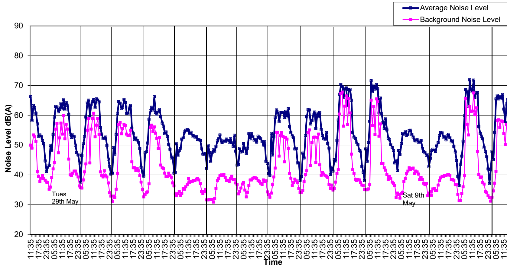
Graph 1: Noise Levels at Location A East Quad West Boundary Wall from 28 th May to 12 th June 2018.
