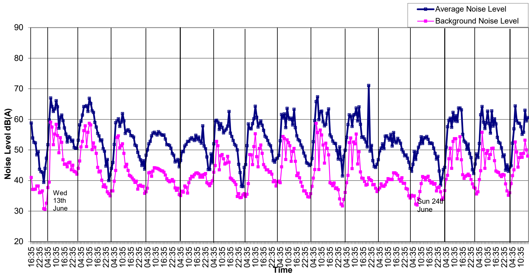
Graph 2: Noise Levels at Location A East Quad West Boundary Wall from 12 th to 27 th June 2018.
