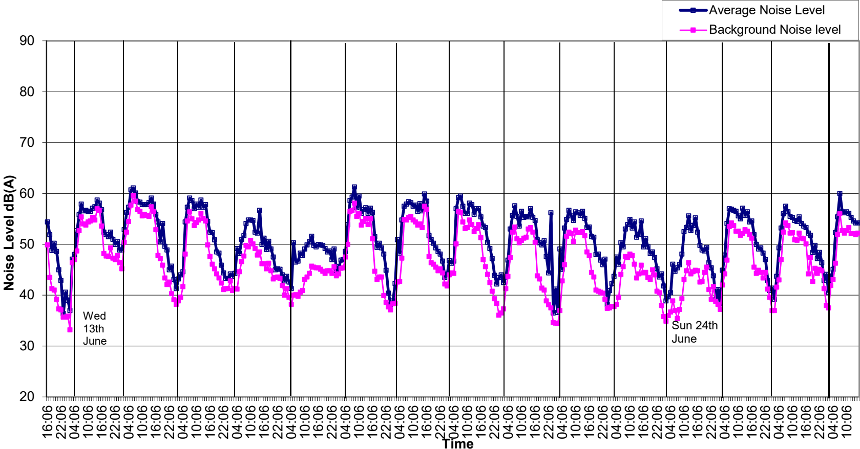
Graph 4: Noise Levels at Location B Grangegorman Upper from 12 th to 27 th June 2018.
