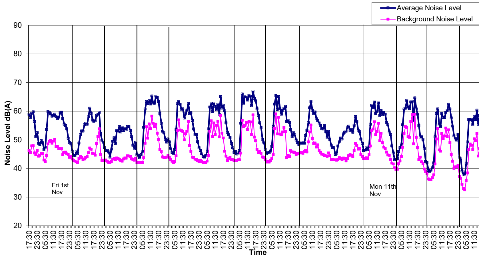
Graph 1: Noise Levels at Location A East Quad West Boundary Wall from 31 st October 14 th November 2019.
