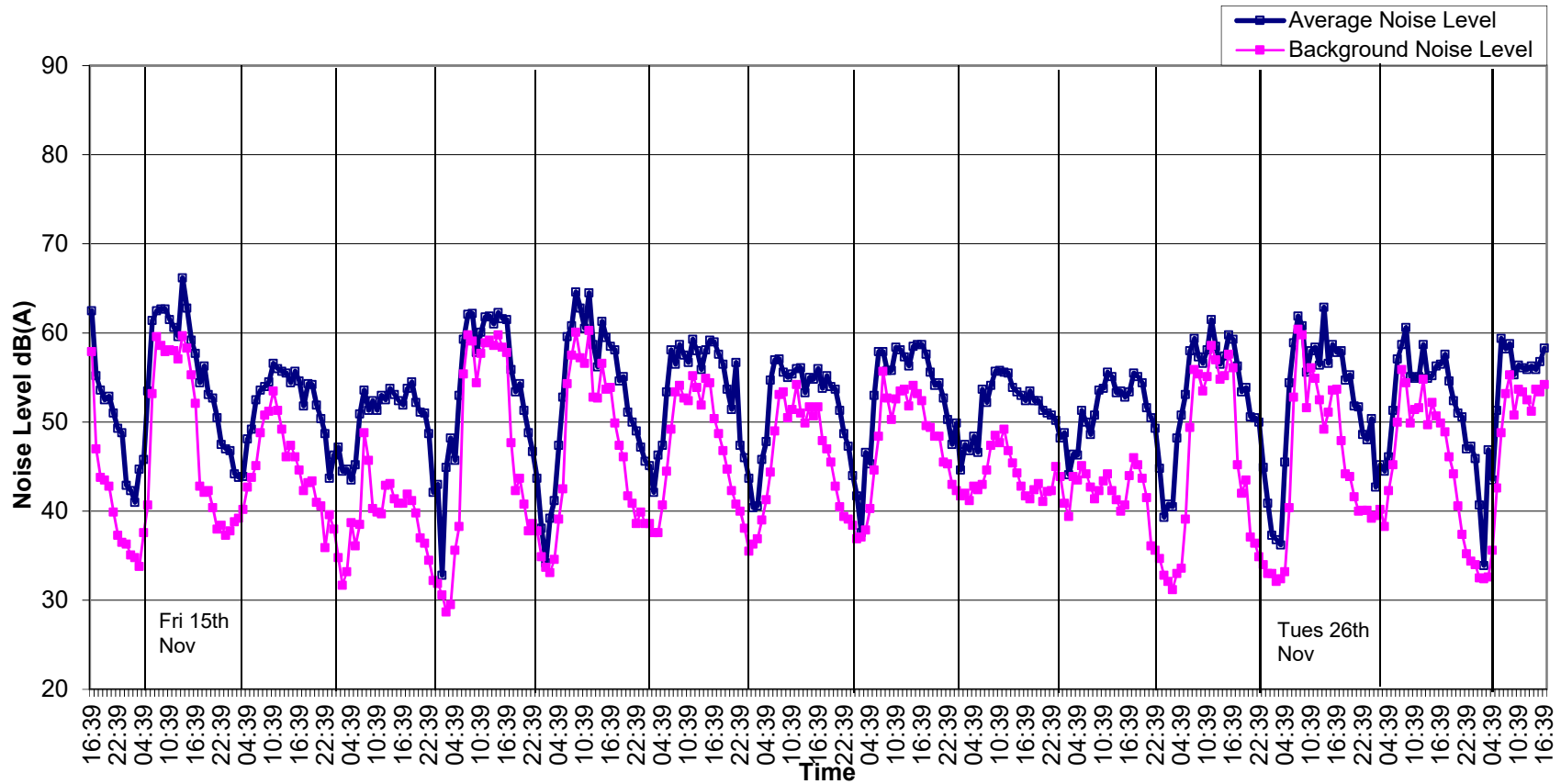
Graph 4: Noise Levels at Location B Grangegorman Upper from 14 th to 28 th November 2019.
