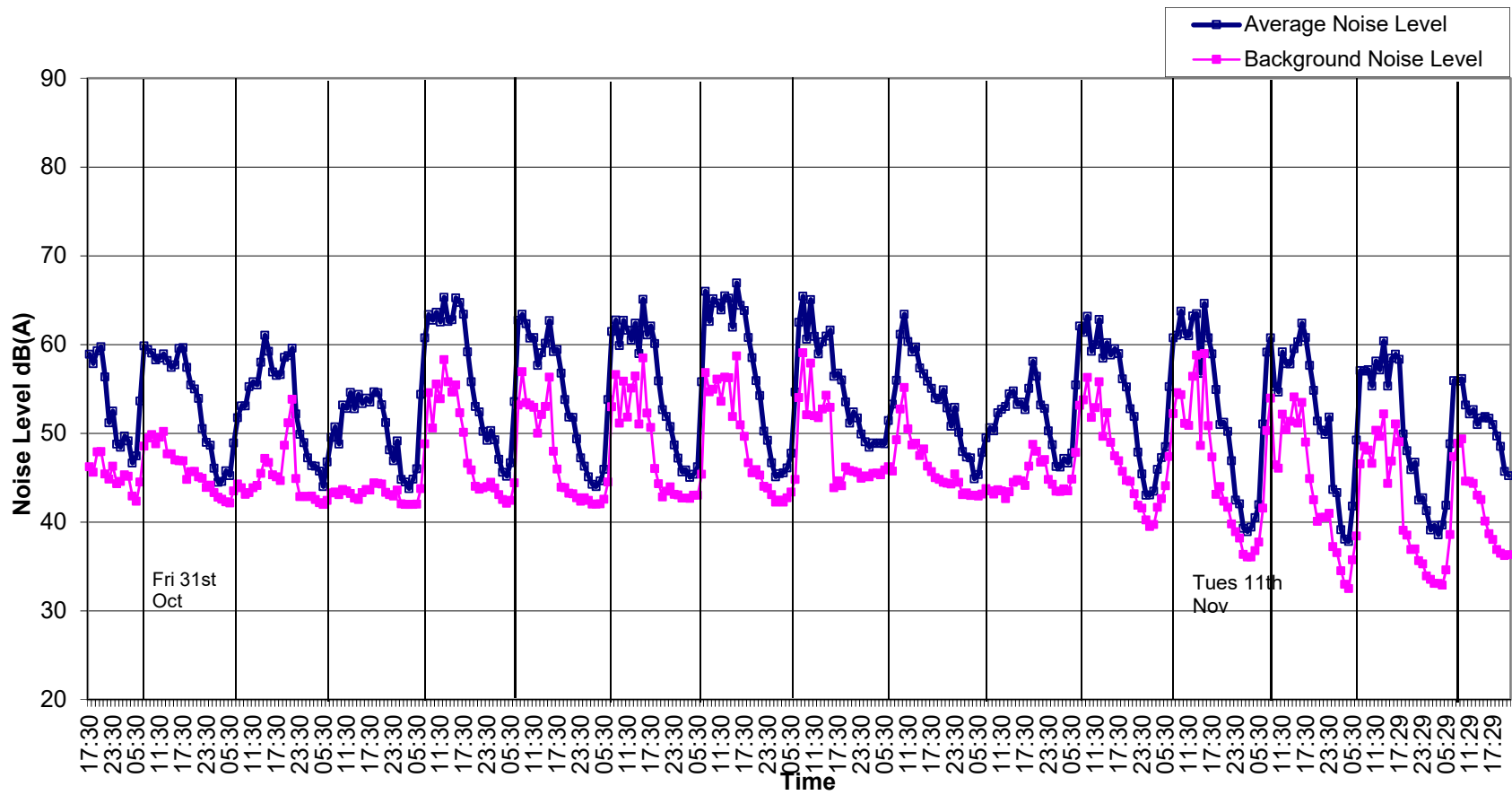
Graph 3: Noise Levels at Location B Grangegorman Upper from 31 st October to 14 th November 2019.
