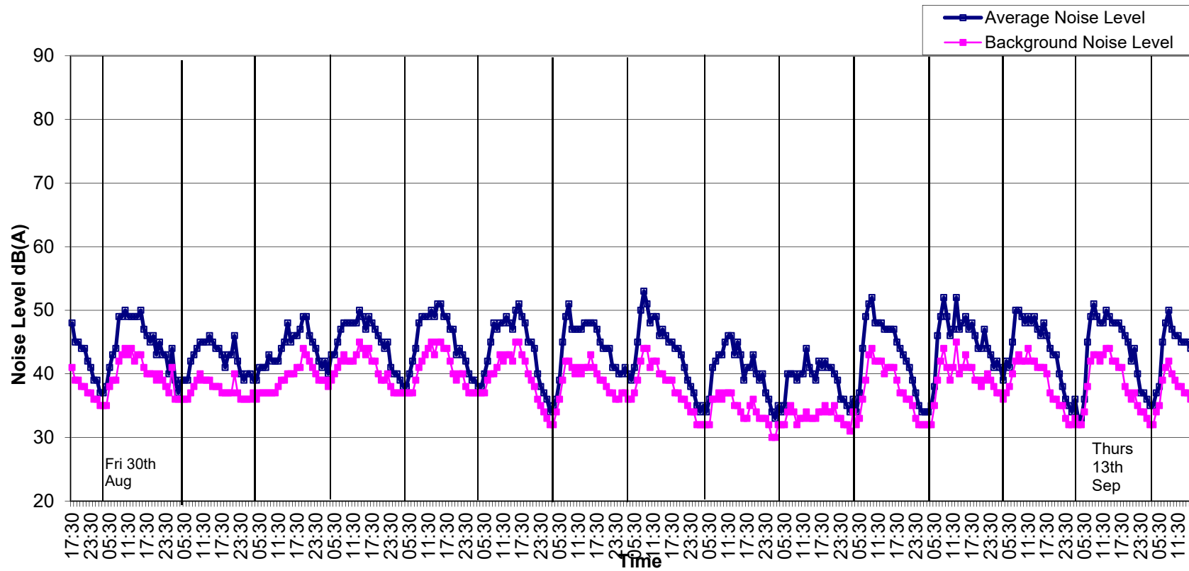
Graph 1: Noise Levels at Location A East Quad West Boundary Wall from 29 th August to 13 th September 2019.
