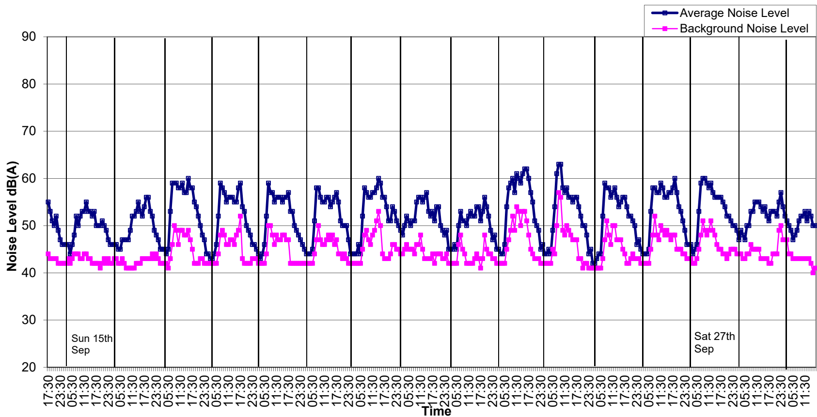
Graph 4: Noise Levels at Location B Grangegorman Upper from 13 th to 29 th September 2019.
