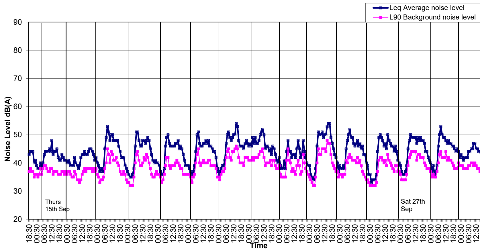
Graph 2: Noise Levels at Location A East Quad West Boundary Wall from 13 th to 29 th September 2019.
