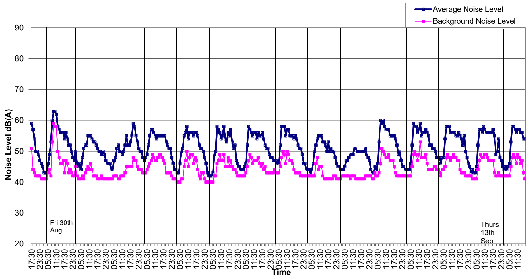
Graph 3: Noise Levels at Location B Grangegorman Upper from 29 th August to 13 th September 2019.
