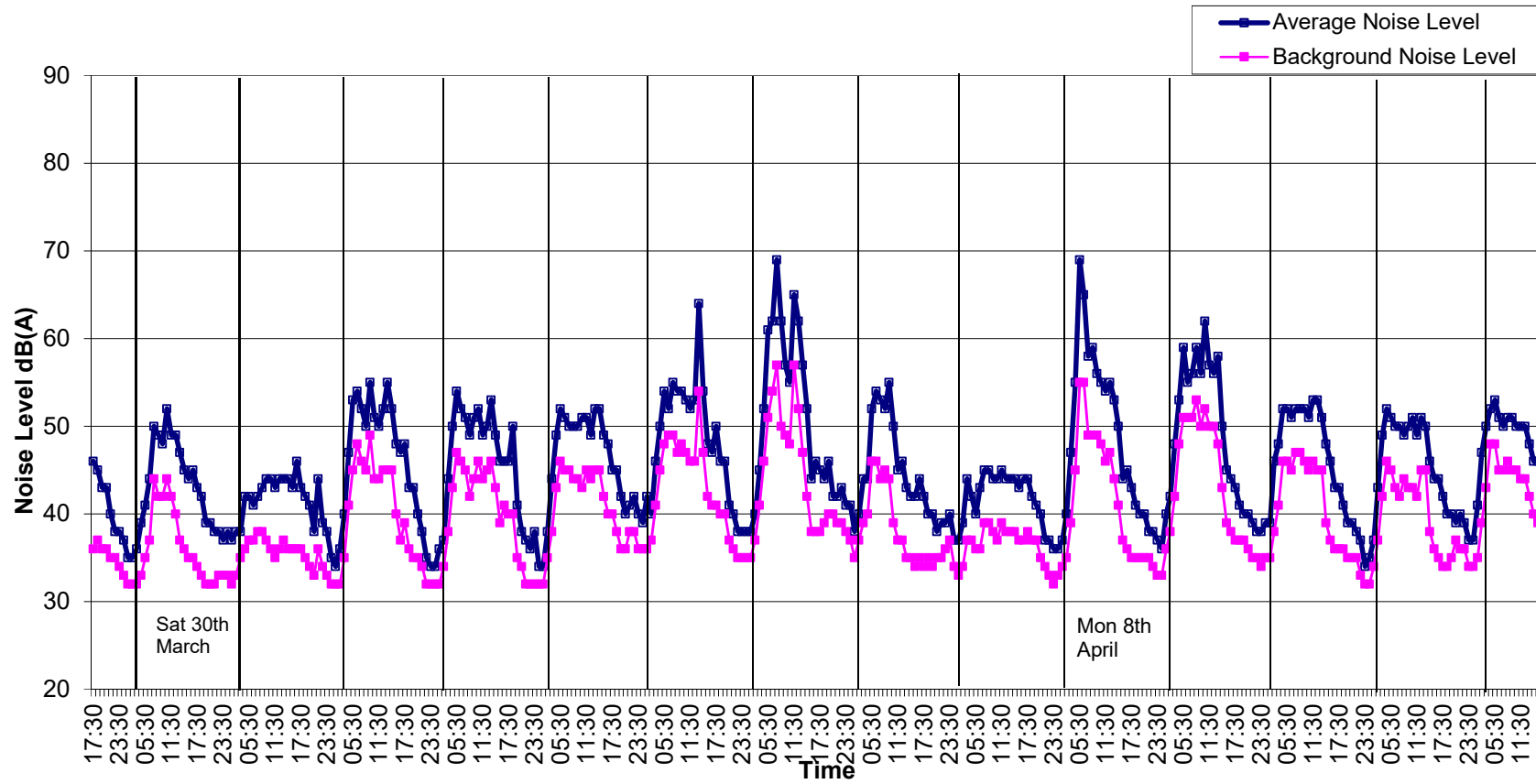
Graph 3: Noise Levels at Location B Grangegorman Upper from 29 th March to 12 th April 2019.
