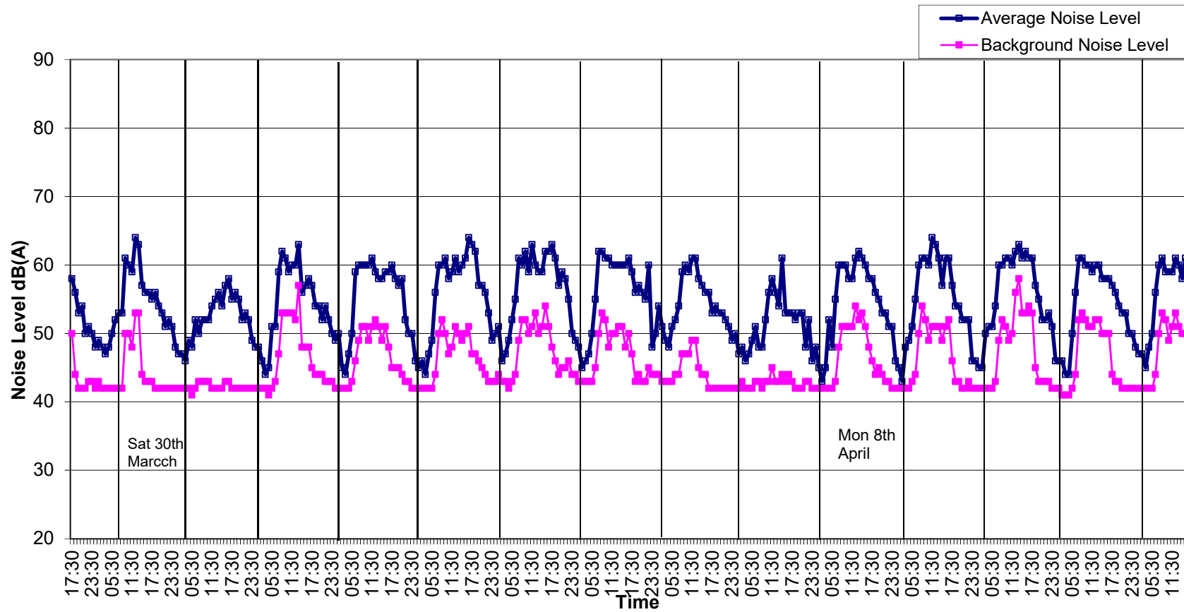
Graph 1: Noise Levels at Location A East Quad West Boundary Wall from 29 th March to 12 th April 2019.
