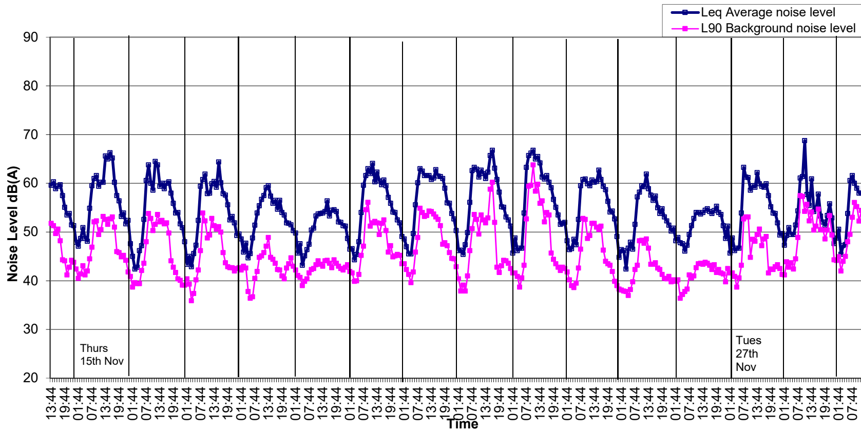
Graph 4: Noise Levels at Location B Grangegorman Upper from 14 th to 29 th November 2018.
