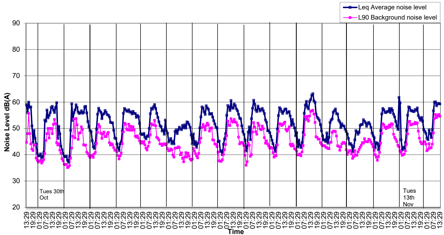
Graph 1: Noise Levels at Location A East Quad West Boundary Wall from 29 th October to 14 th November 2018.
