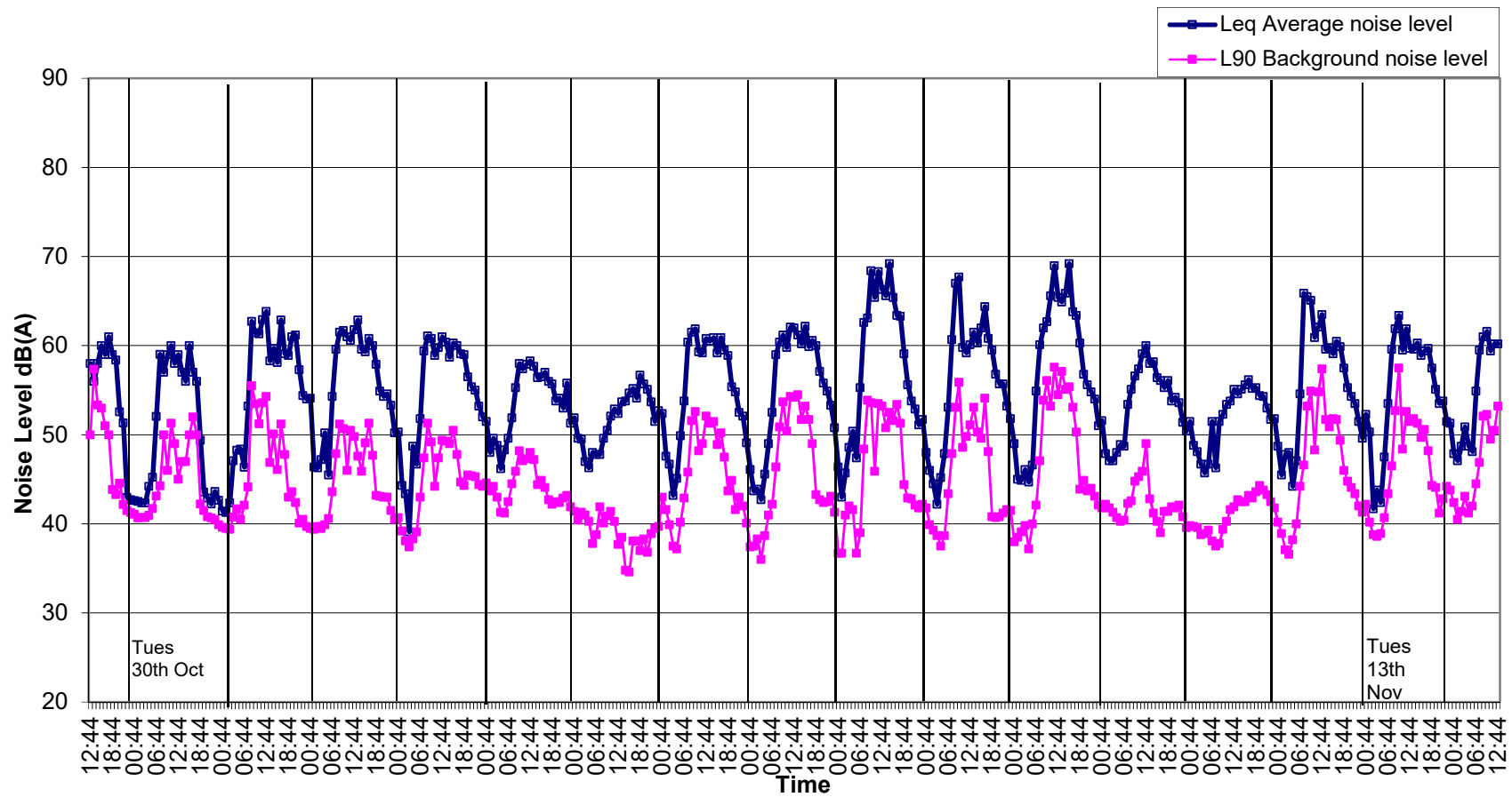
Graph 3: Noise Levels at Location B Grangegorman Upper from 29 th October to 14 th November 2018.
