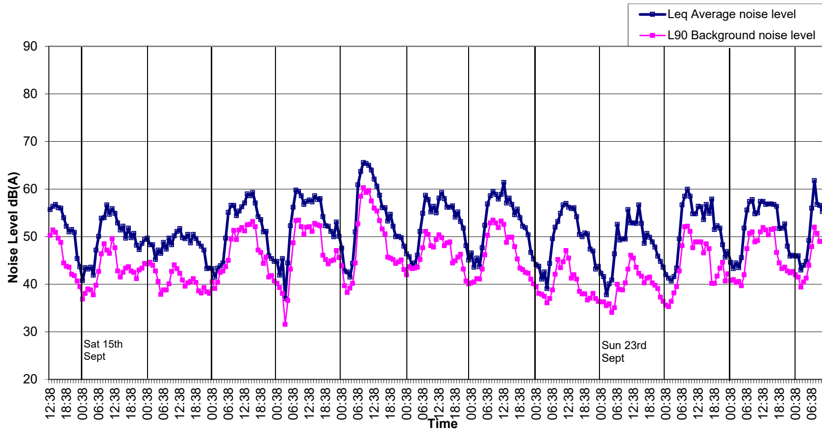
Graph 4: Noise Levels at Location B Grangegorman Upper from 14 th to 26 th September 2018.
