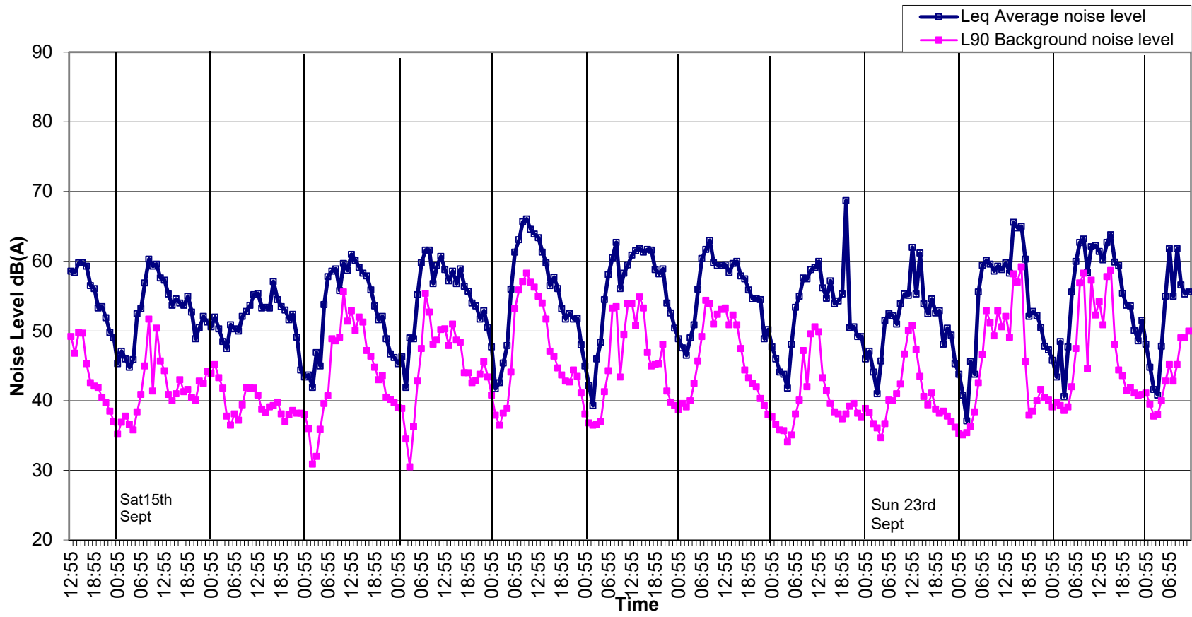
Graph 2: Noise Levels at Location A East Quad West Boundary Wall from 14 th to 26 th September 2018.
