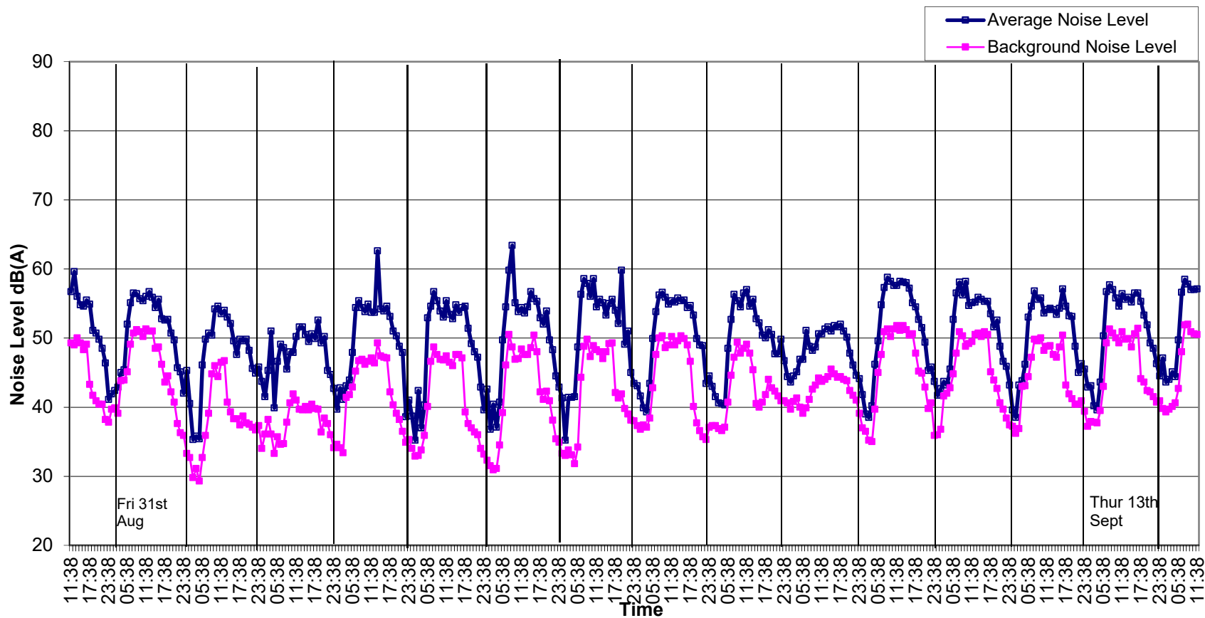
Graph 3: Noise Levels at Location B Grangegorman Upper from 30 th August to 14 th September 2018.
