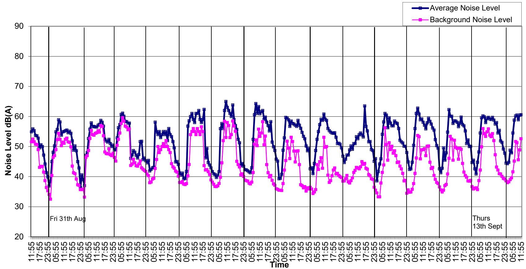
Graph 1: Noise Levels at Location A East Quad West Boundary Wall from 30 th August to 14 th September 2018.
