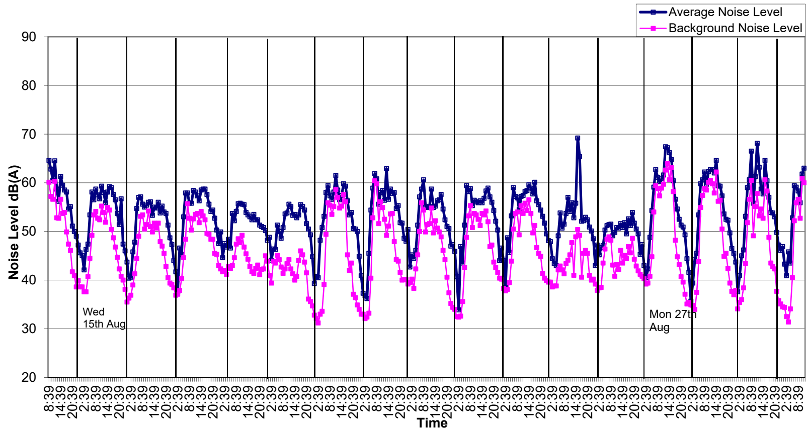
Graph 2: Noise Levels at Location A East Quad West Boundary Wall from 14 th to 30 th August 2018.
