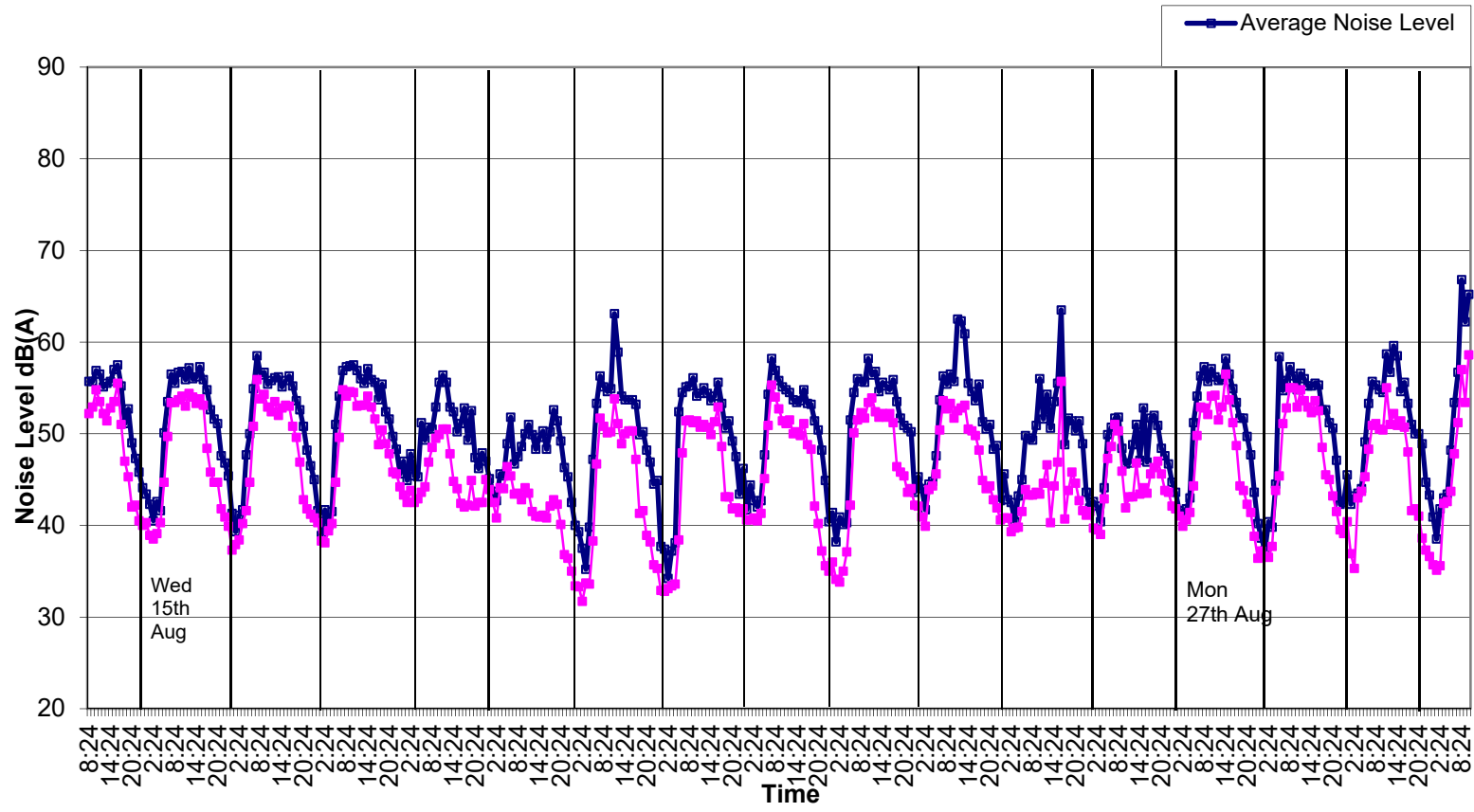
Graph 4: Noise Levels at Location B Grangegorman Upper from 14 th to 30 th August 2018.
